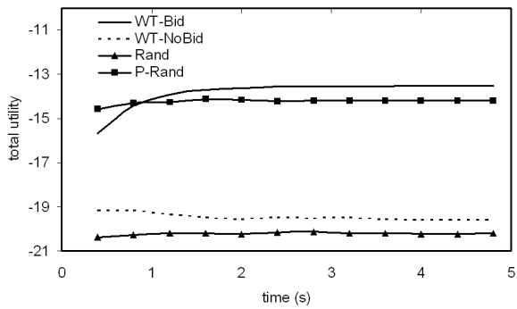
(a) Average of total utility
