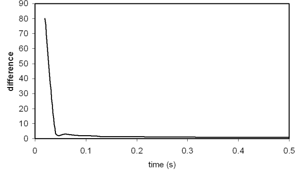
Fig. 1: Convergence of the weighted transmission policy
