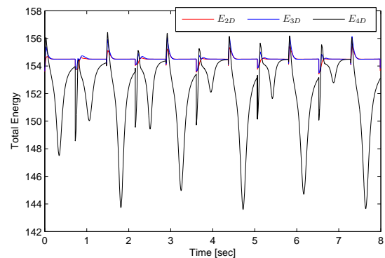
Fig. 4. Subsystem energies of the hipped 4-d.o.f. biped's 90^\circ -turn gait.
