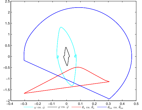
Fig. 2. Phase portrait of the 4-d.o.f. biped's straight-walking limit cycle.
