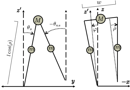
Fig. 1. The sagittal and lateral planes of a three-dimensional bipedal robot.
